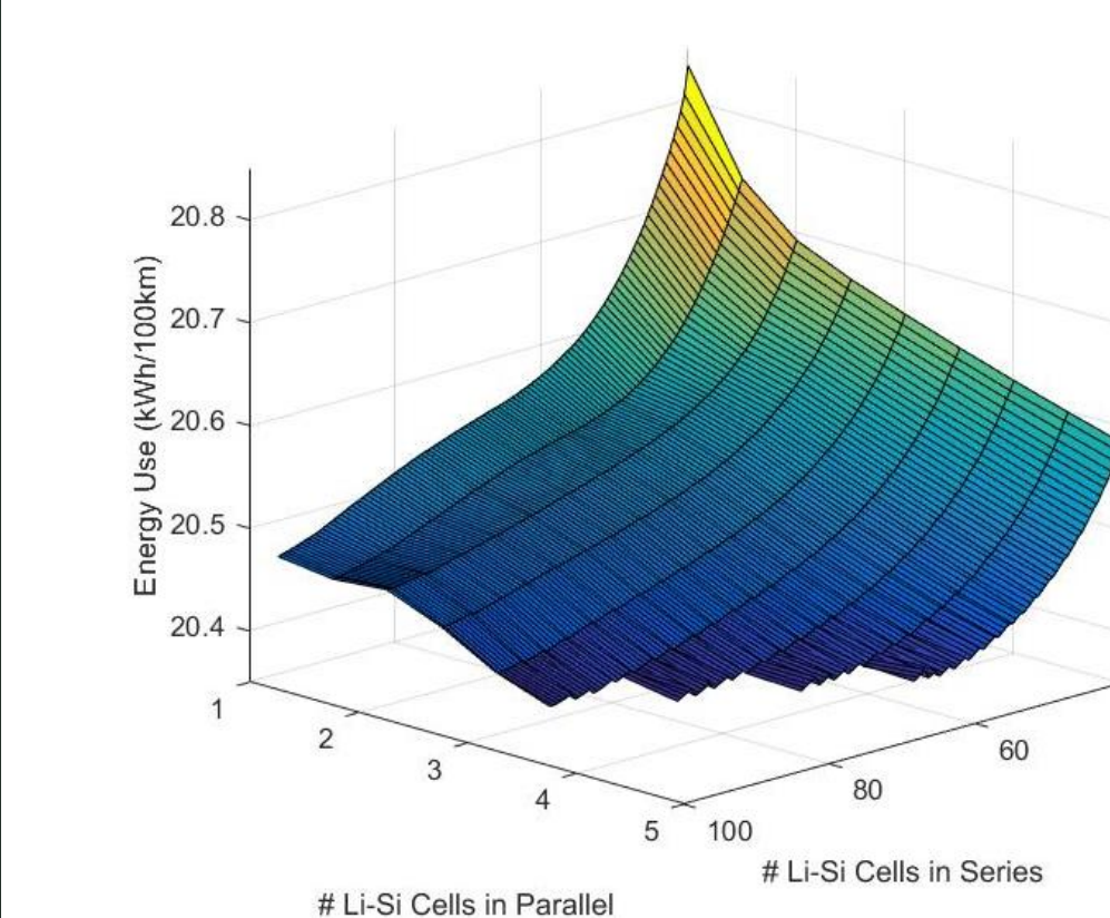
Topology 1 Energy Use
