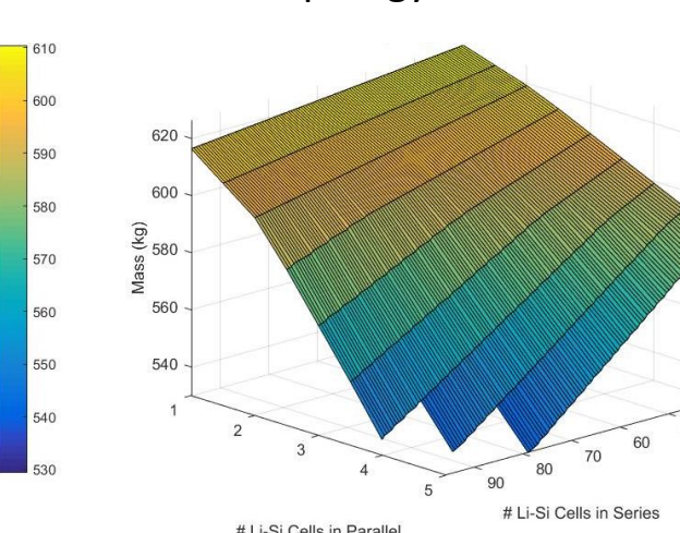
Topology 2 HESS Mass
