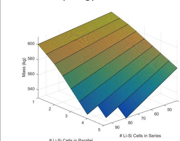
Topology 1 HESS Mass
